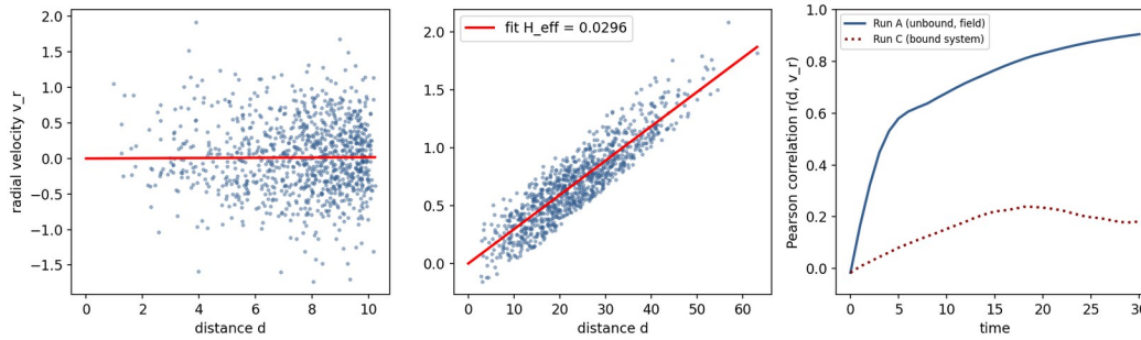
Radial velocity against distance at t=0 (no correlation) and at t=30 after gravitational sorting ( r=0.904 ), with the growth of the correlation over time in Run A and Run C.
